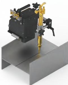
Beam Splitting
